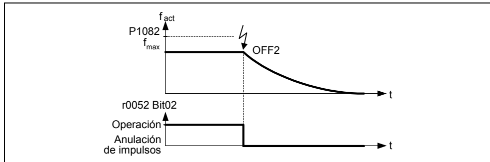
Figura 3-45 OFF2
