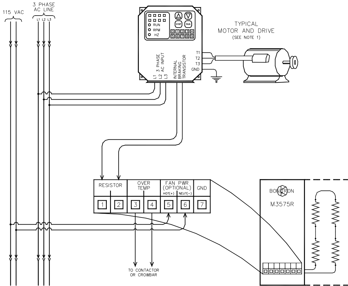
Figure 3-2: Typical Braking Resistor Field Connections
