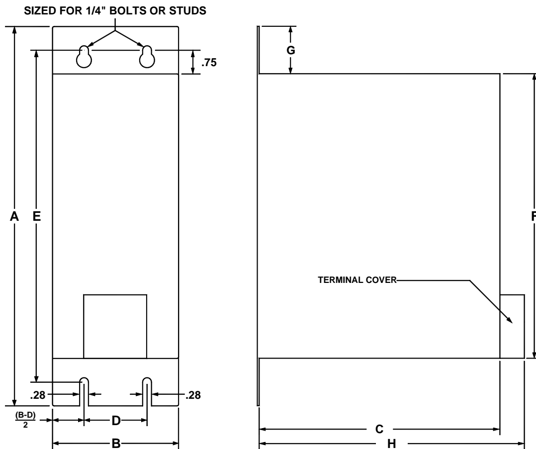
Figure 6-1: Bookshelf and Mini Chassis Dimensional Outline Drawing
