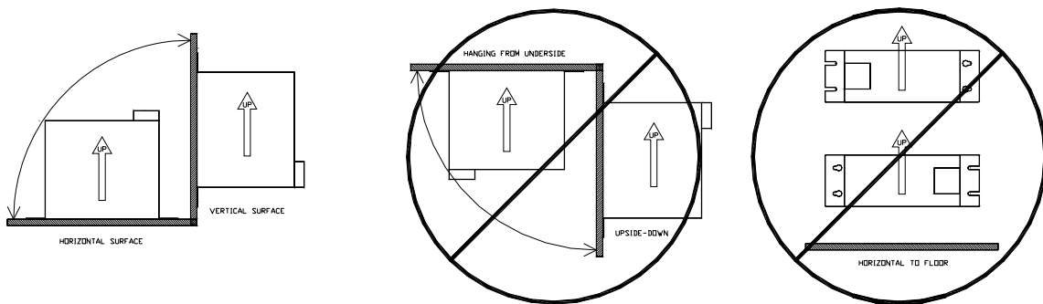
Figure 3-1: M3575R Mounting Orientation
