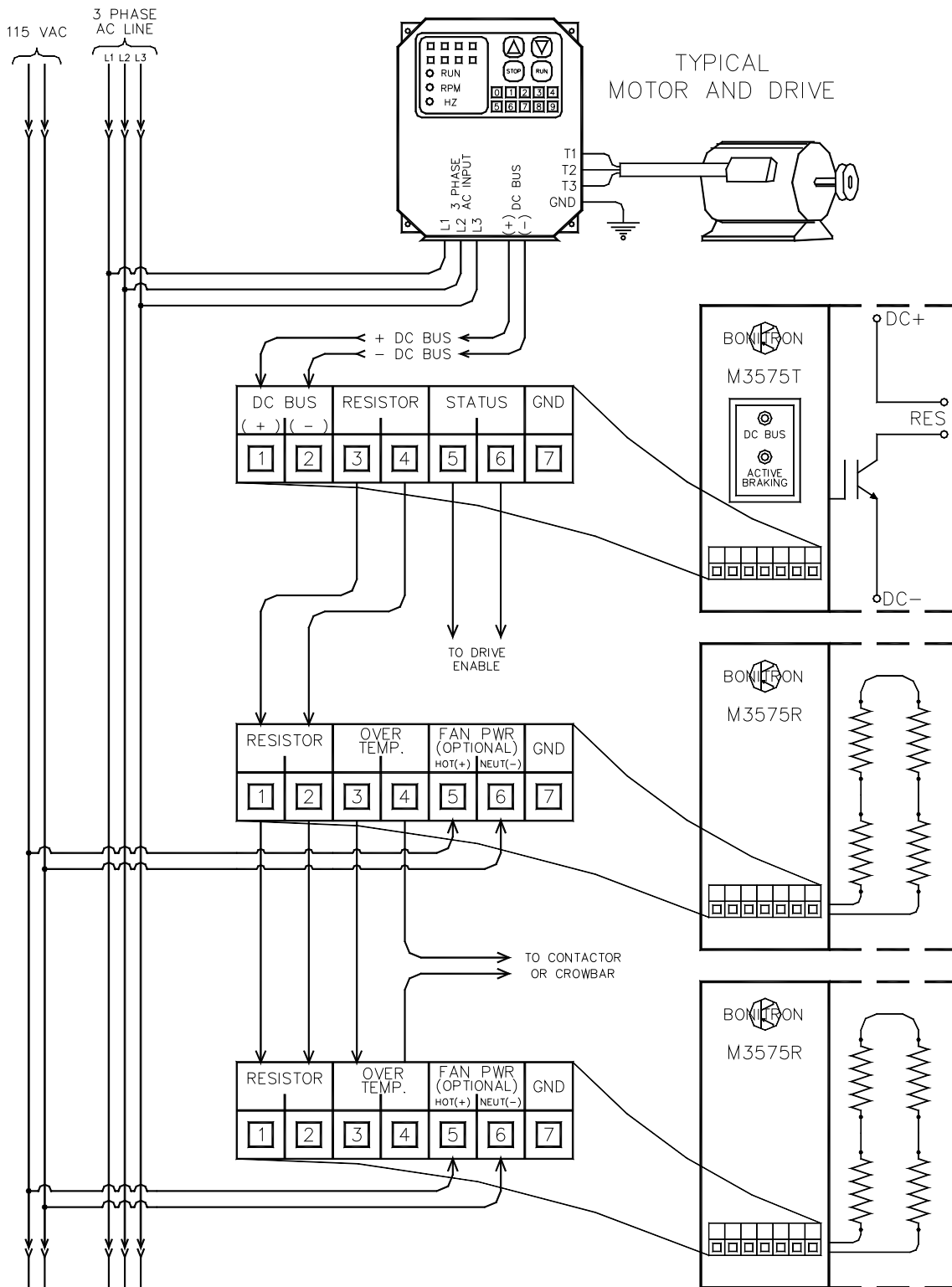
Figure 3-4: Typical Braking Interconnection Diagram With Parallel Load Modules
